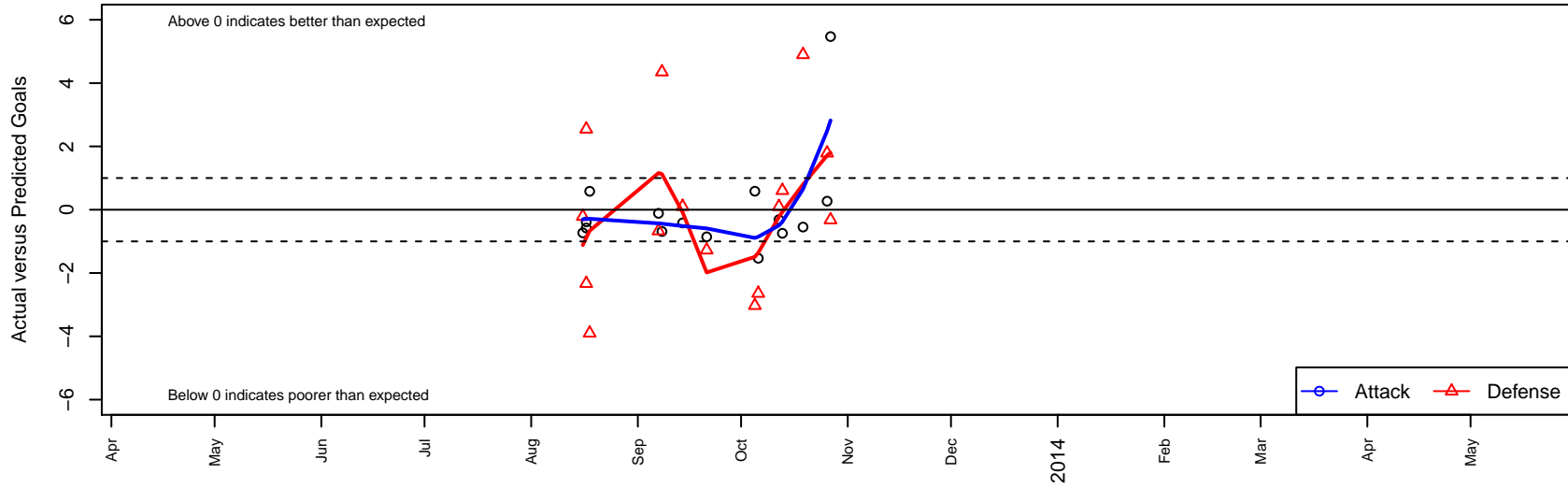
Foothills SC Lumberjacks B99 Dots are actual minus expected GF (blue circles) and GA (red triangles). Blue line is smoothed change in attack strength. Red is smoothed change in defense strength.
